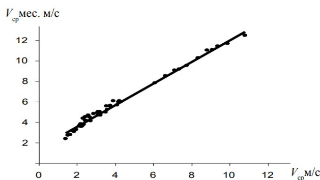
Figure 2. Dependence of the energy characteristics of the wind flow on the average wind speed
